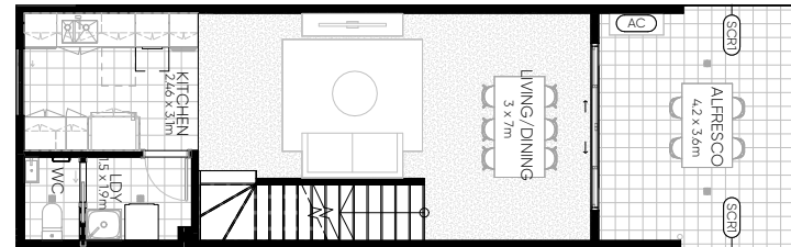
LEVEL 1
