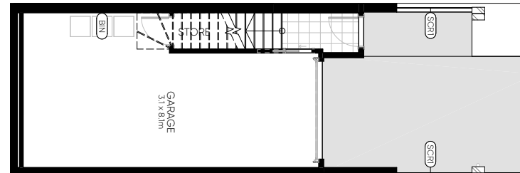
GROUND
