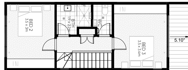
LEVEL 2
