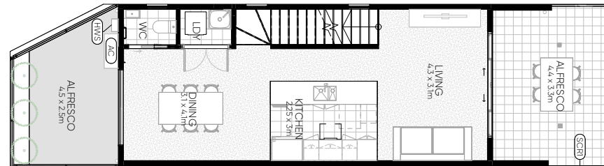
LEVEL 1
