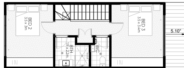
LEVEL 2
