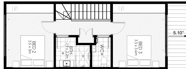
LEVEL 2
