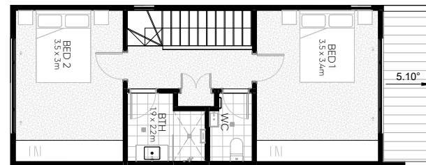
LEVEL 2
