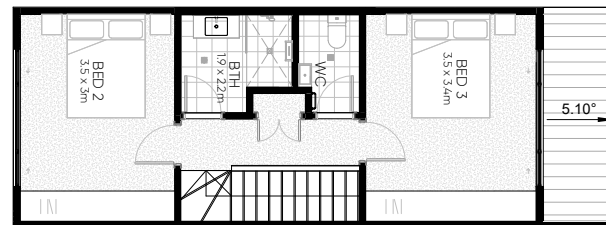
LEVEL 2
